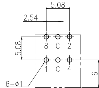
P.C.B DIMENSION (Top View)
